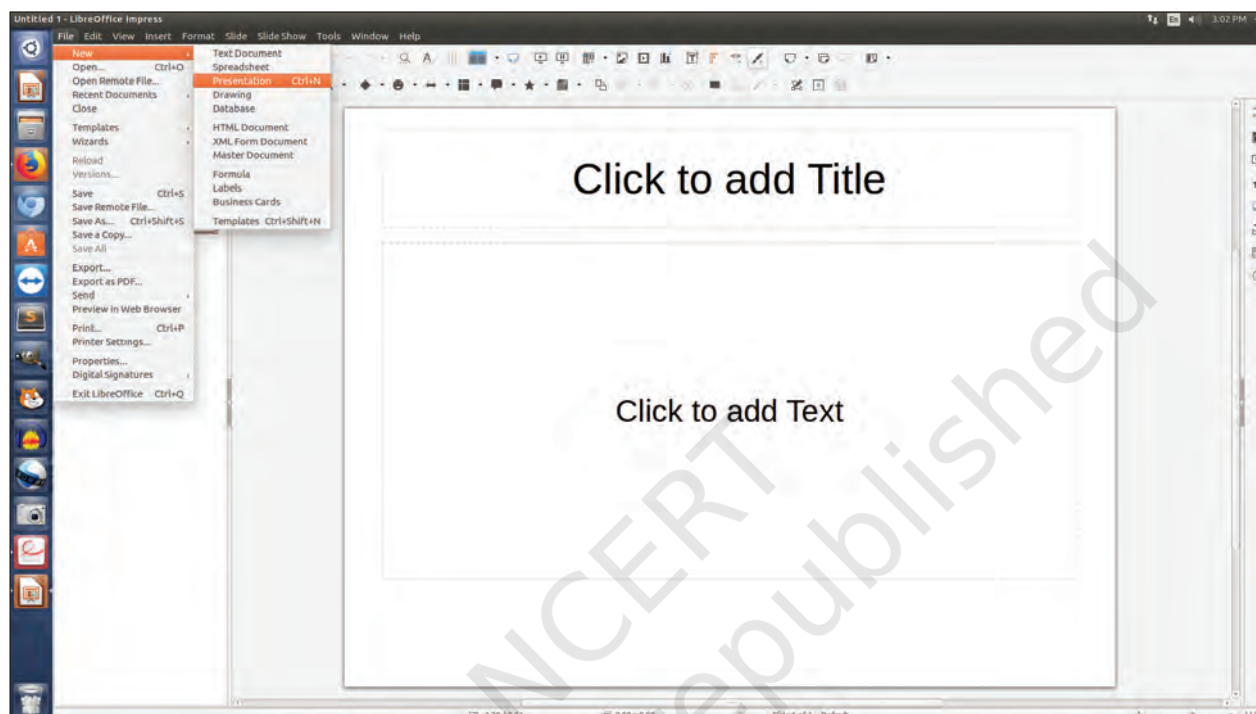
Fig. 5.1: Impress interface
