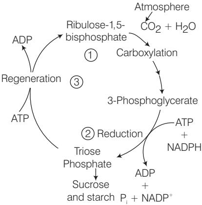
Calvin cycle
