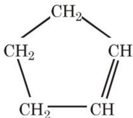
Cyclopentene
