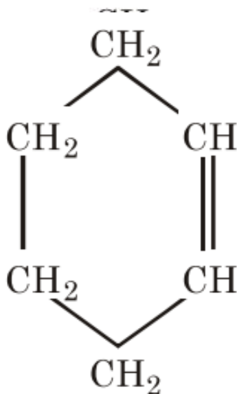
Cyclohexene
