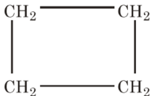
Cyclobutane
