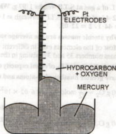
FIGURE 1.6. Eudiometry.
