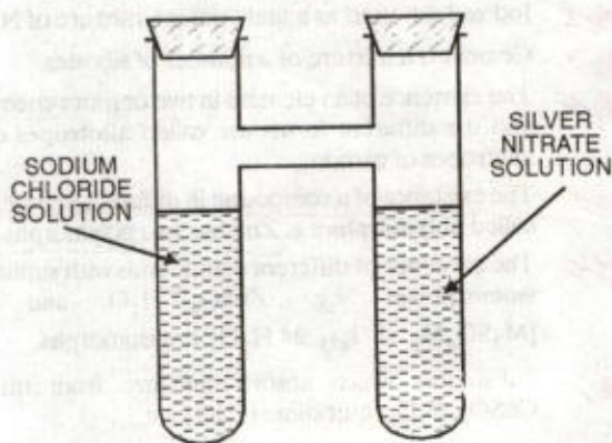
FIGURE 1.2. Landolt's tube.
