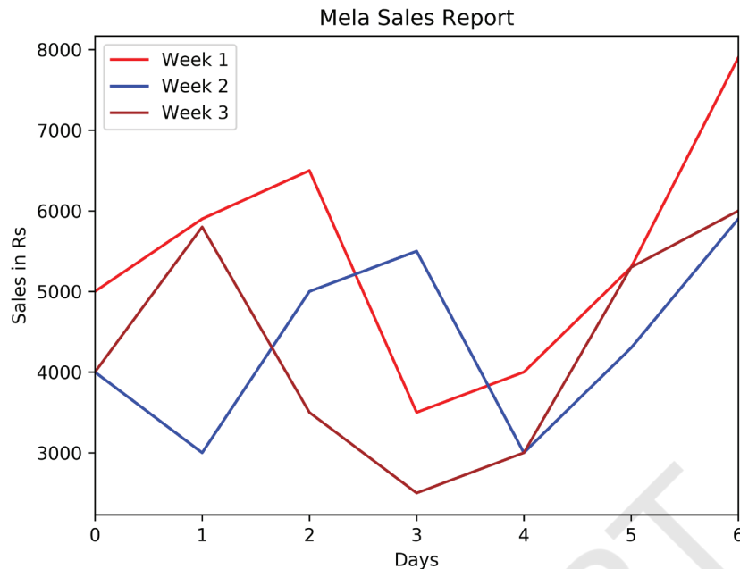
Figure 4.5: Line plot showing mela sales figures
