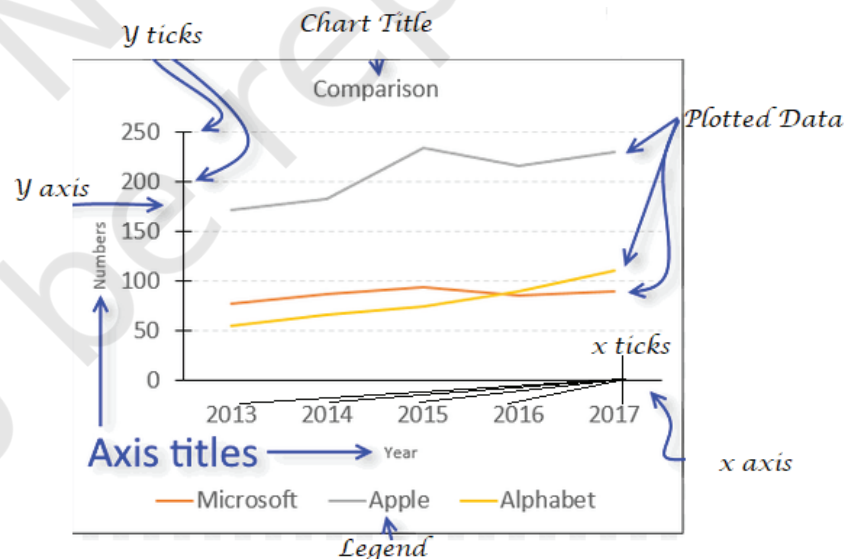
Figure 4.1: Components of a plot
