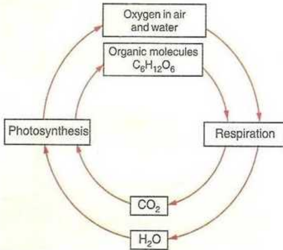
Oxygen cycle.
